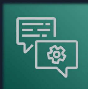
Amazon Lex
