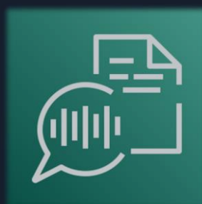
Amazon Transcribe
