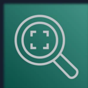
Amazon Rekognition
